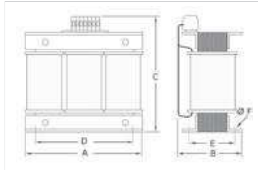
Dimensions TRT 30 IP00
