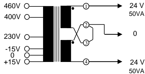
CON TOMA MEDIA WITH MIDDLE TAP
