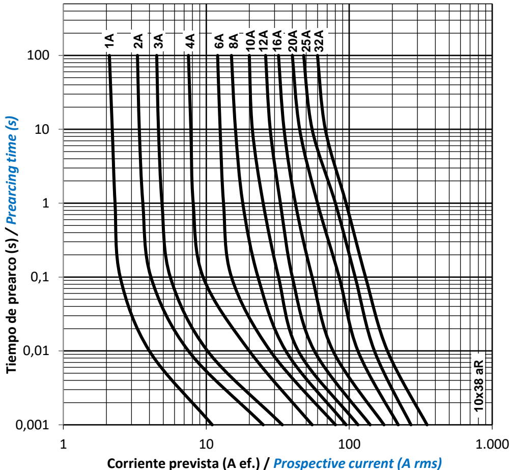
CARACTERÍSTICAS TIEMPO-CORRIENTE TIME-CURRENT CHARACTERISTICS
