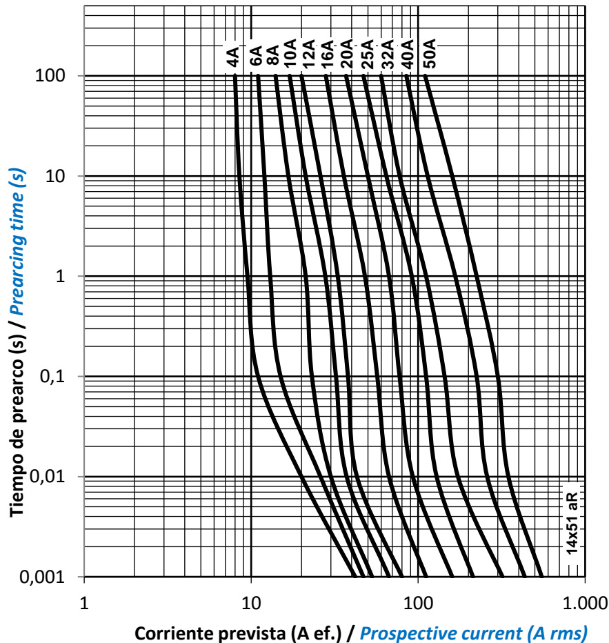
CARACTERÍSTICAS TIEMPO-CORRIENTE TIME-CURRENT CHARACTERISTICS
